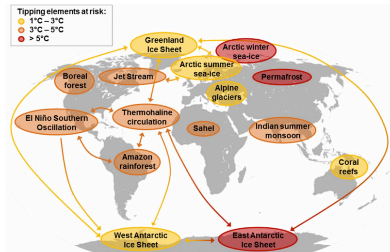
Figure 3. Global map of potential tipping cascades. The individual tipping elements are color-coded according to estimated thresholds in global average surface temperature (tipping points) (12, 34). Arrows show the potential interactions among the tipping elements based on expert elicitation that could generate cascades. Note that, although the risk for tipping (loss of) the East Antarctic Ice Sheet is proposed at >5 °C, some marine-based sectors in East Antarctica may be vulnerable at lower temperatures (35–38).
