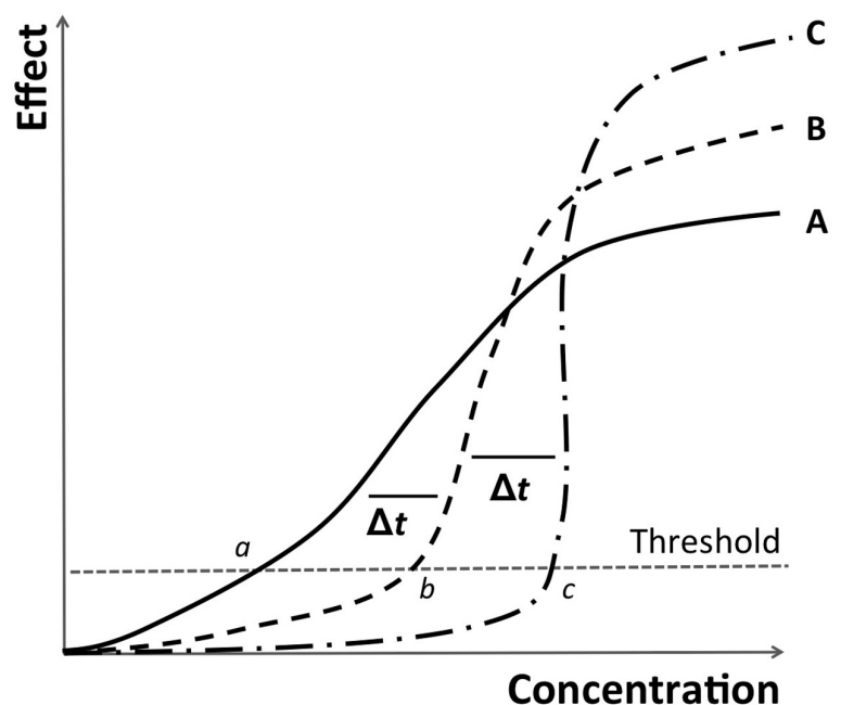
Fig. 2. Cross-scale spatial and temporal dynamics of marine plastic pollution. A. Effect on organisms – direct ‘local’ effects, observed all around the world. Threshold a set normatively as a precautionary boundary (e.g., maximum acceptable exposure of populations). B. Effect on ecosystems – large-region, time-lagged ( \Delta t ) effects. Threshold b reflects a structural ecosystem-level shift (e.g., loss of keystone species). C. Cascading effect on global ecosystem function (e.g., globalised toxic bioaccumulation impacts on genera or families). Minimal effect seen until critical ecosystem shift (c) occurs.
